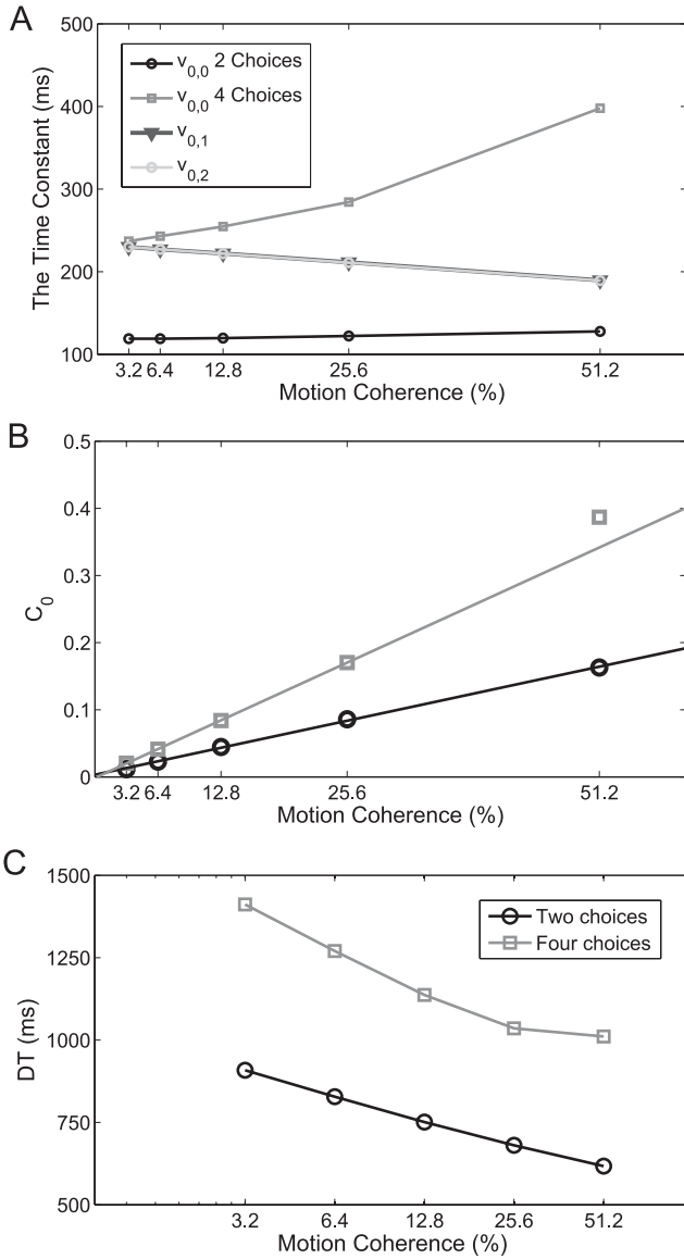
Figure 10: Approximation of the reaction time. (A) The time constants of the system are defined by the reciprocal of the largest positive eigenvalue of the unstable steady state \tilde{S}_{u,1} . (B) The projection coefficient, c_0 , for two- and four-choice decision making increases with the coherence level of the motion stimuli. (C) Approximated reaction time (see formula 4.6) for two- and four-choice decision making.
