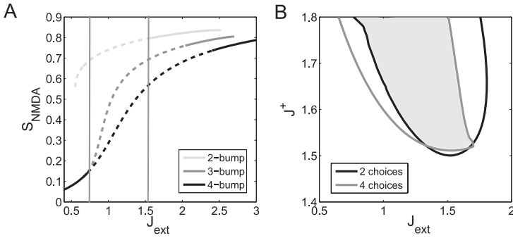
Figure 9: Parameter ranges of the network supporting decision making. (A) The peak of the highest bump of the unstable steady states \bar{S}_{u,1} , \bar{S}_{u,2} , and \bar{S}_{u,3} as a function of the external input strength J_{ext} for four choices. Solid (dashed) lines indicate that the corresponding states are stable (unstable). The parameter in the interval between two vertical lines supports a decision. (B) The overlapping parameter domains for two- and four-choice decision making. The parameter ranges supporting decisions are enveloped by the dark curve for two choices and the gray curve for four choices.
